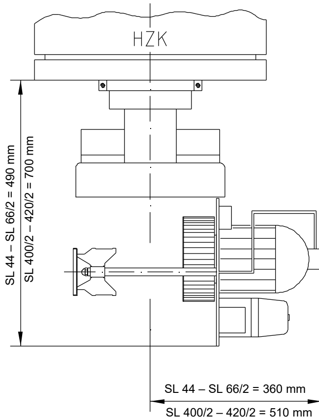
Abb. 19: Brenner in Serviceposition
