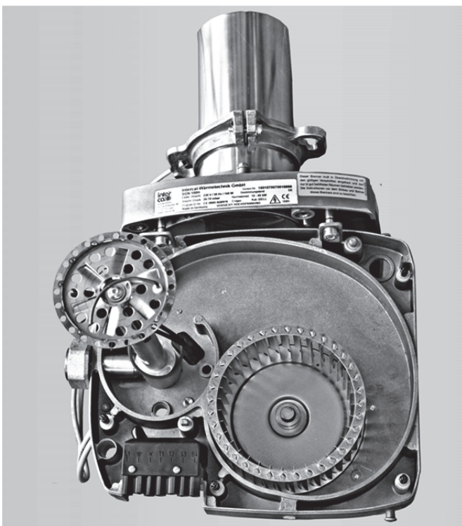
Abb. 16: Serviceposition
